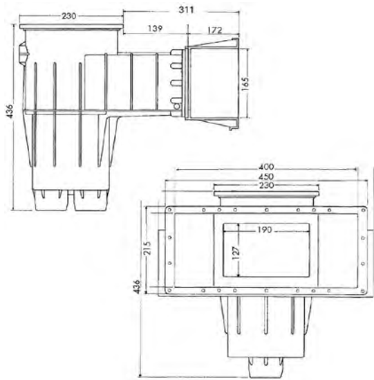
Skimmer brede opening 04.6205, 04.6207 en 04.6206
