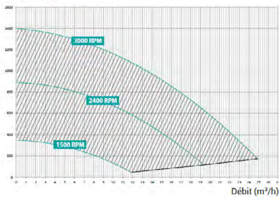
Curve 1PK
