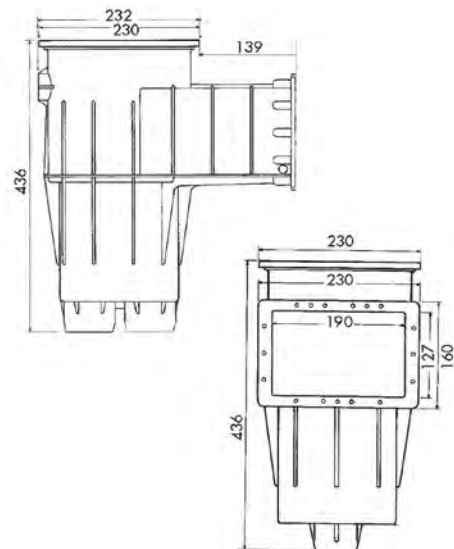
Skimmer kleine opening 04.6200, 04.6202 en 04.6201
